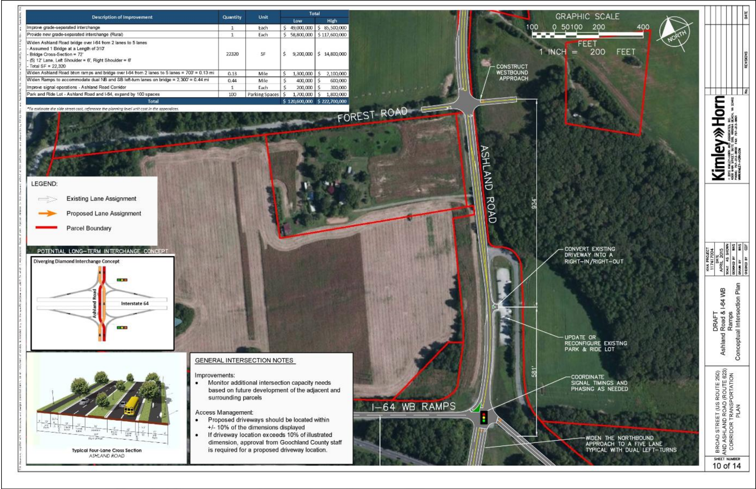
Plan Sheet 10: AMP Recommendations – Ashland Road at WB I-64 Ramps
