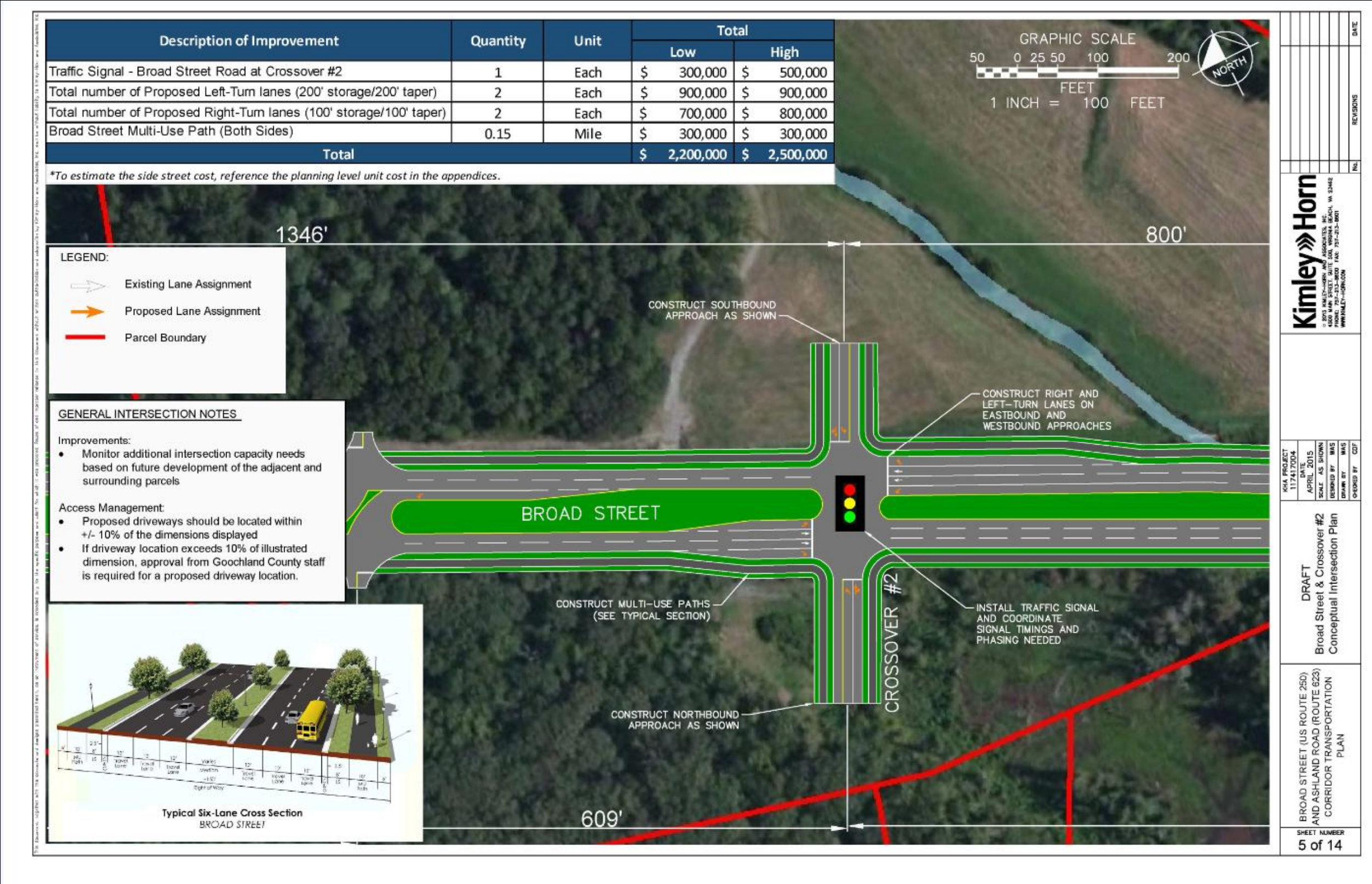
Plan Sheet 5: AMP Recommendations – Broad Street at Crossover #2
