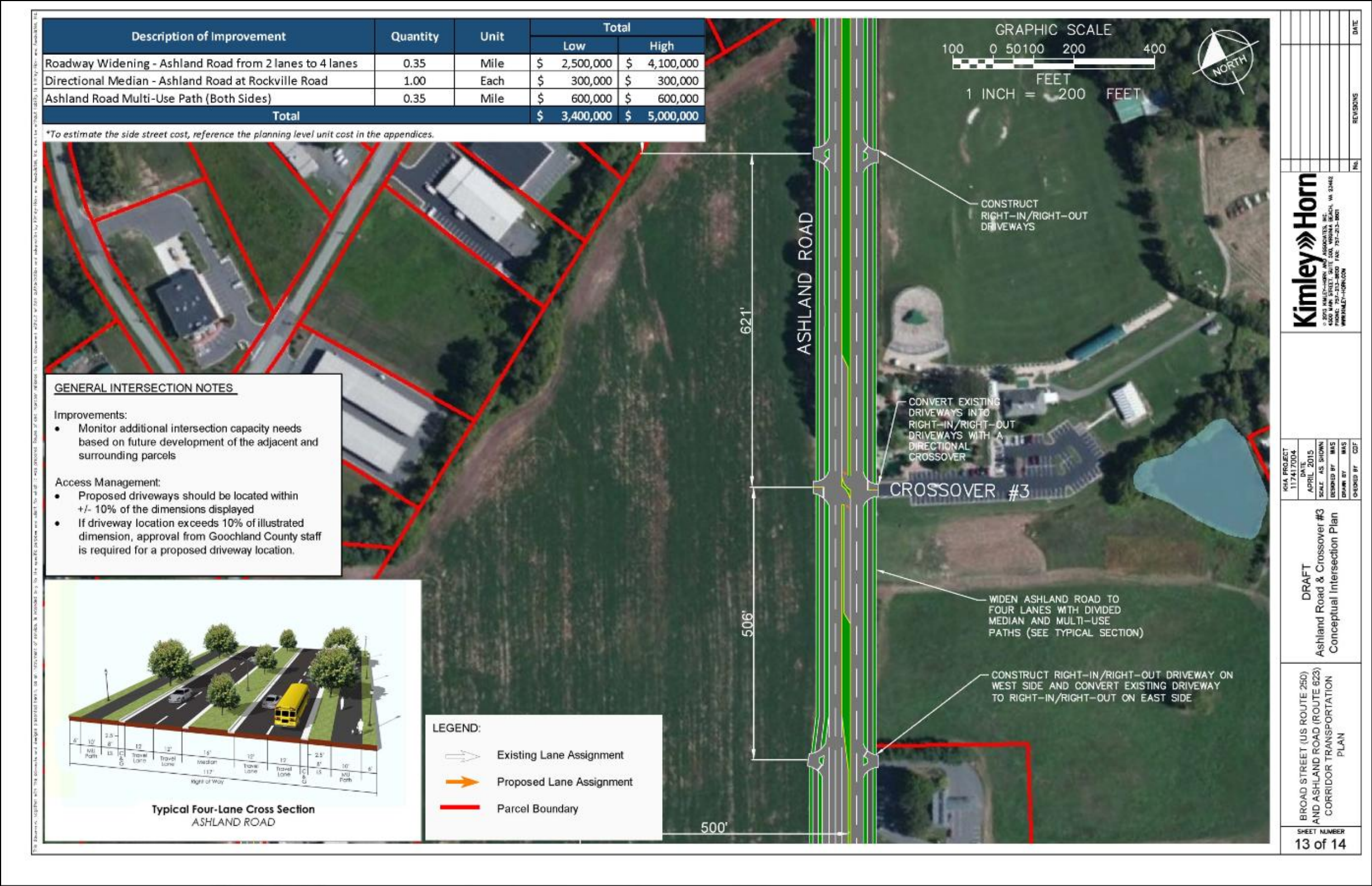
Plan Sheet 13: AMP Recommendations – Ashland Road at Crossover #3
