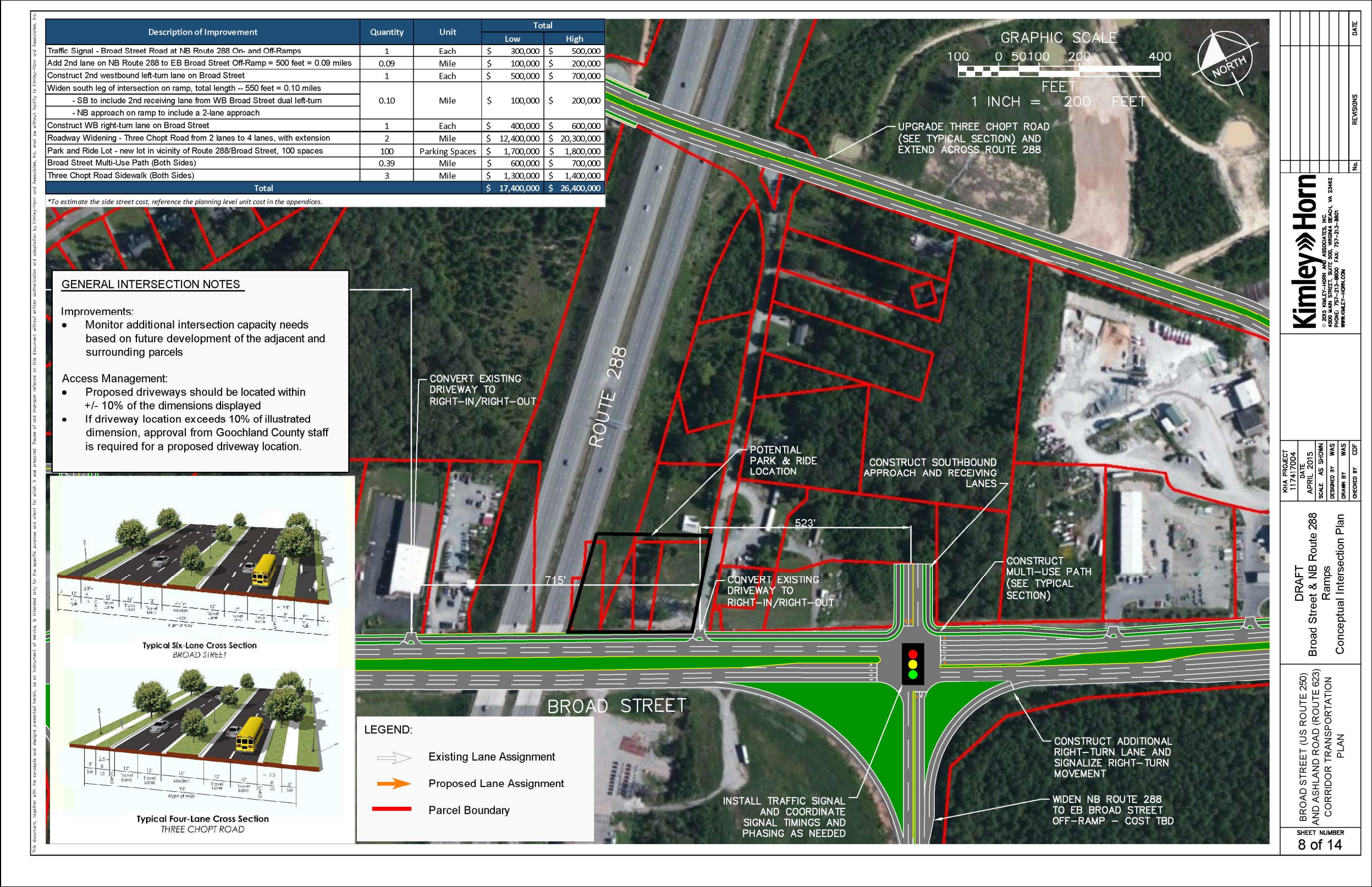
Plan Sheet 8: AMP Recommendations – Broad Street at NB Route 288 Ramps
