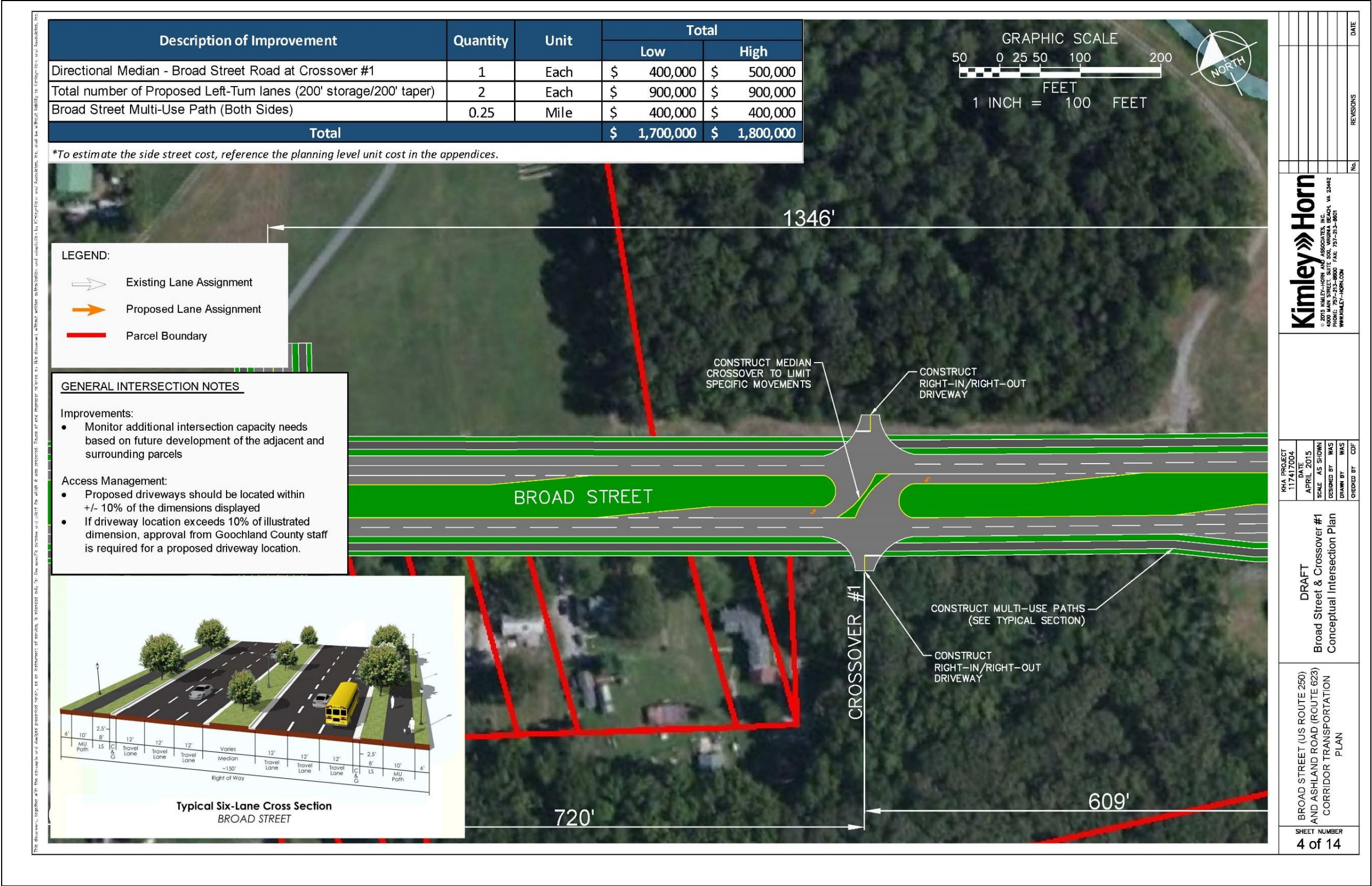
Plan Sheet 4: AMP Recommendations – Broad Street at Crossover #1
