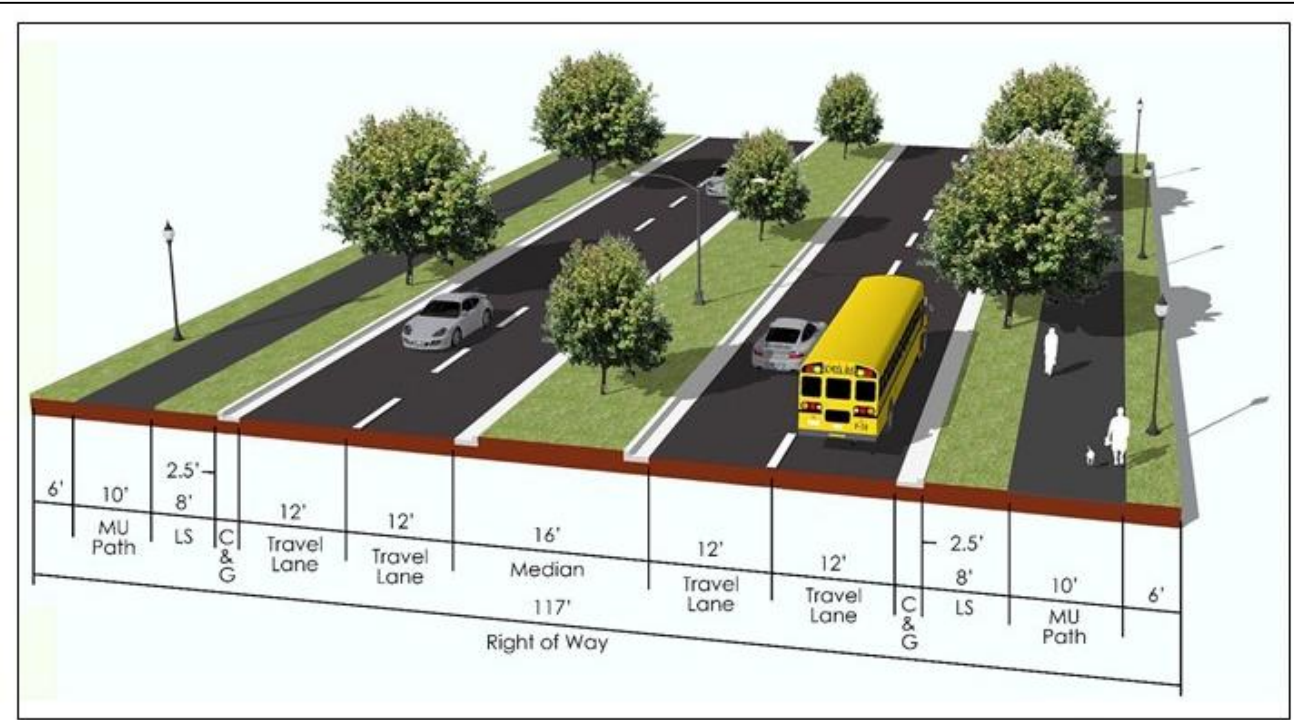
Typical Four-Lane Cross Section – Ashland Road Arterial Management and Interstate Access Plan
