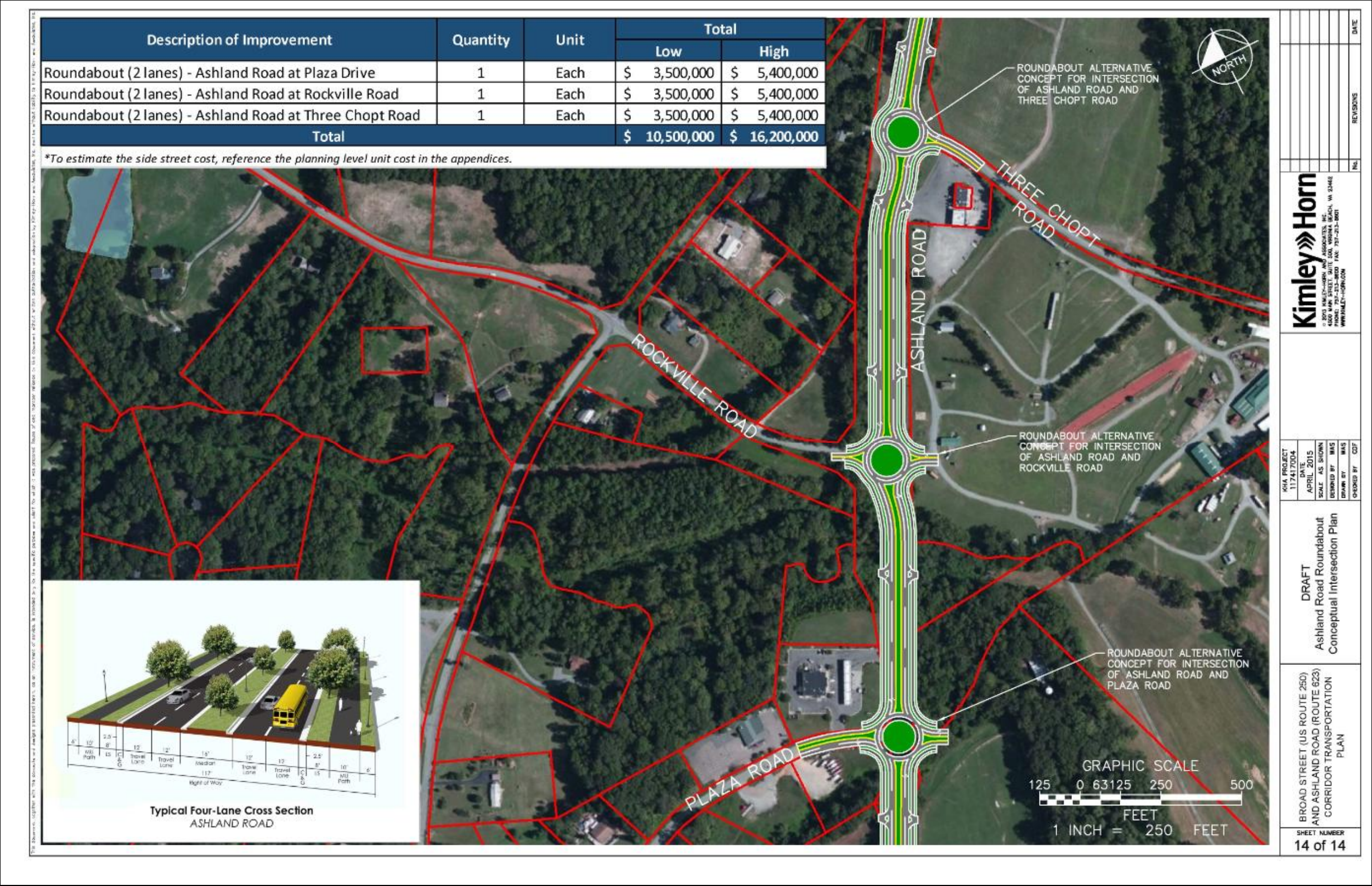
Plan Sheet 14: AMP Recommendations – Ashland Road Potential Roundabout Locations
