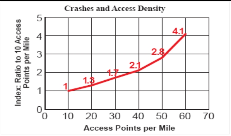
Composite Crash Rate Indexes 2
