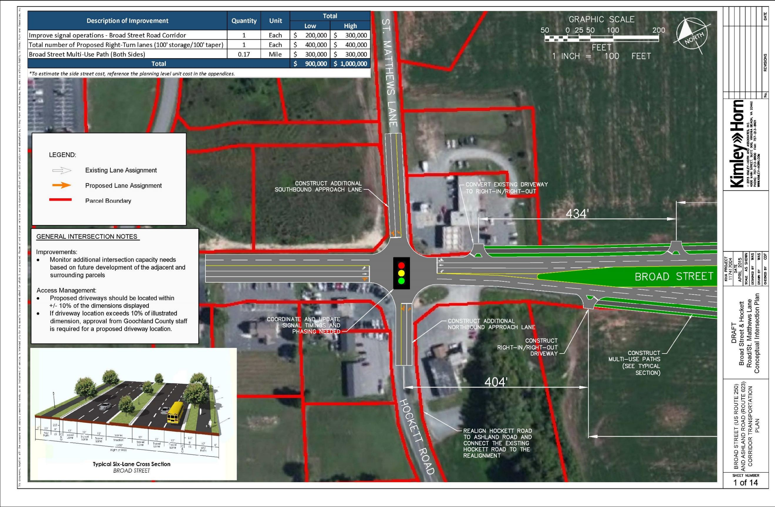
Plan Sheet 1: AMP Recommendations – Broad Street at Hockett Road
