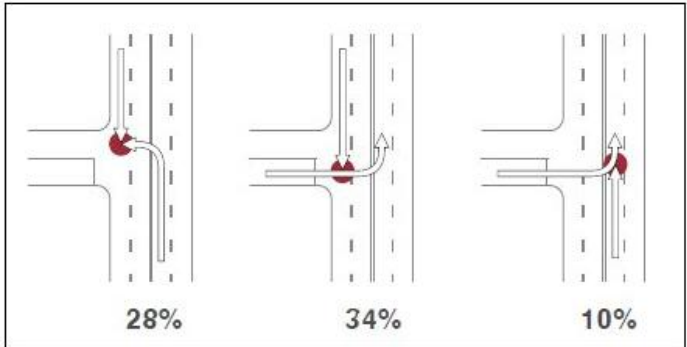
Crash Percentages for Left-Turning Motorists to and from a Driveway 3
