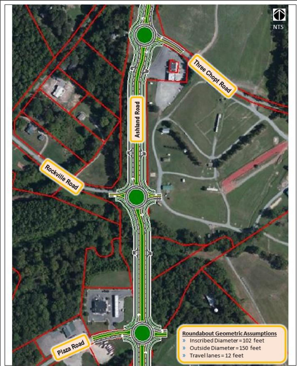
Conceptual Layout of Potential Roundabout Locations Arterial Management and Interstate Access Plan
