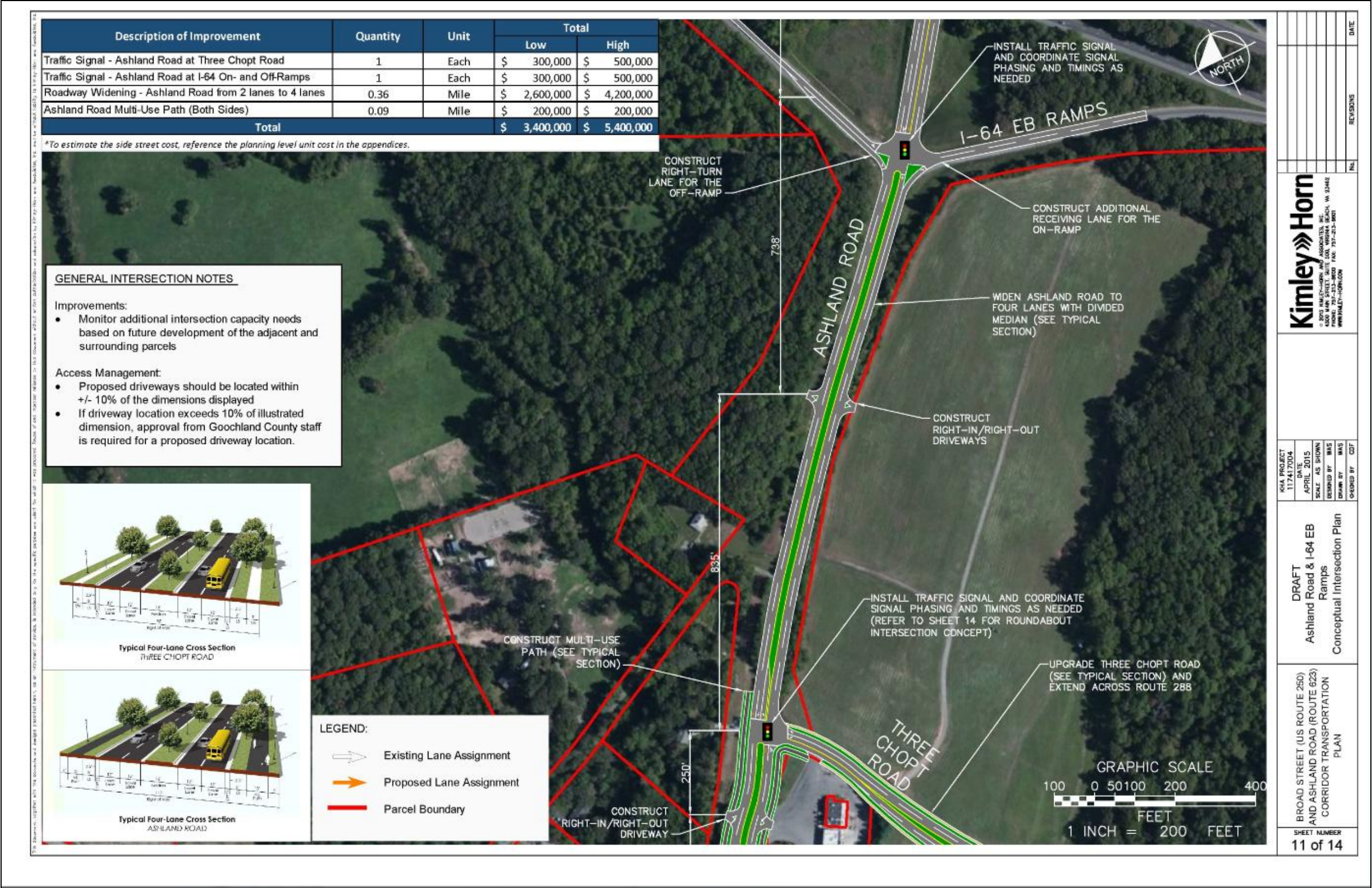
Plan Sheet 11: AMP Recommendations – Ashland Road at EB I-64 Ramps
